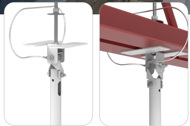
The Wren by 3Si Telescopic Ceiling Mount System
